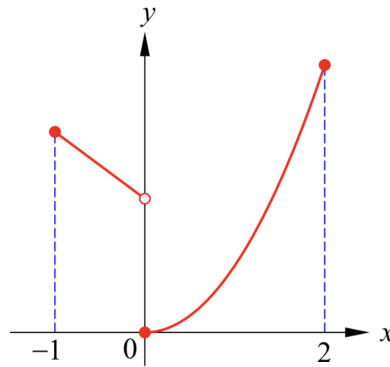
Figure 4.8: The piecewise continuous function defined in Example 4.15.
