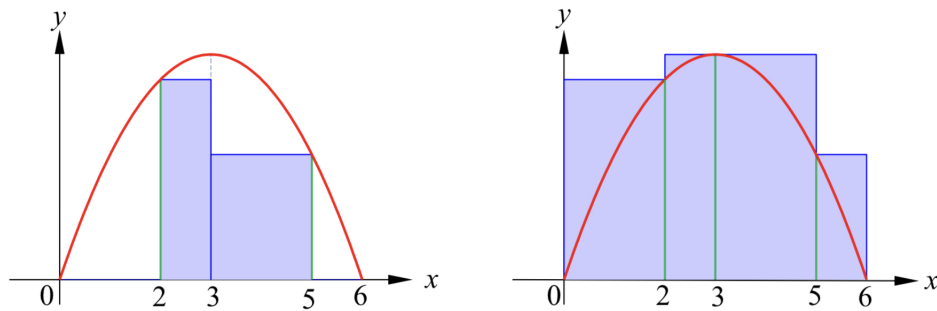
Figure 4.3: Darboux lower sum and Darboux upper sum.
