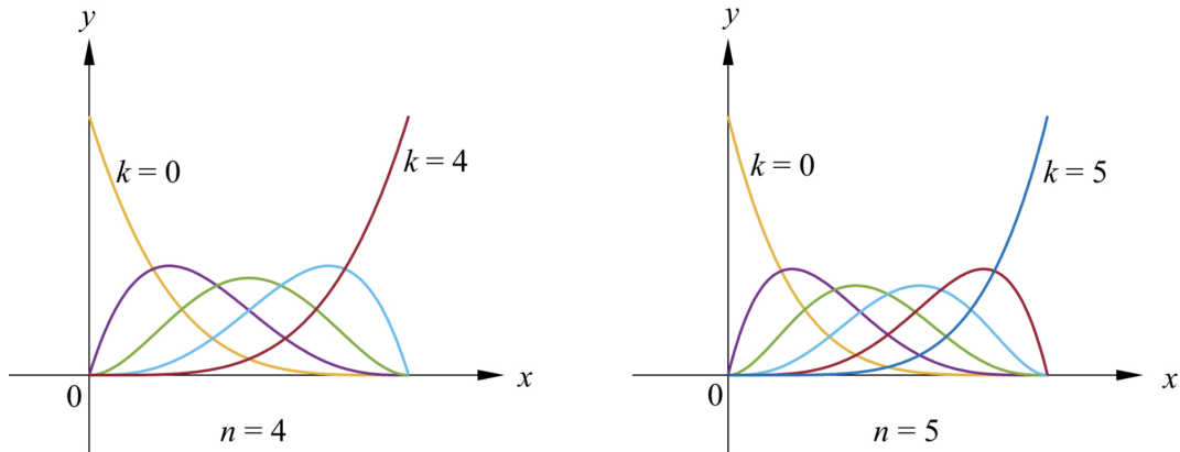
Figure 6.15: The polynomials p_{n,k}(x) = \binom{n}{k} x^k (1-x)^{n-k} when n = 4 and n = 5 , for all 0 \leq k \leq n .
